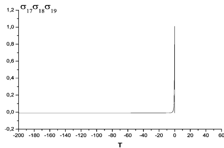
Figure 7: AM \sigma_{17}\sigma_{18}\sigma_{19} after rotating.
