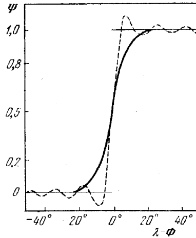
Figure 2: Comparison of Ferraz-Mello and Lala-Sehnal approximation.
