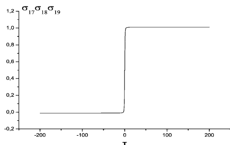
Figure 8: AM \sigma_{17}\sigma_{18}\sigma_{19} combination of last two.
