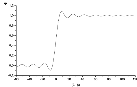
Figure 4: Fourier's series with 20 terms.
