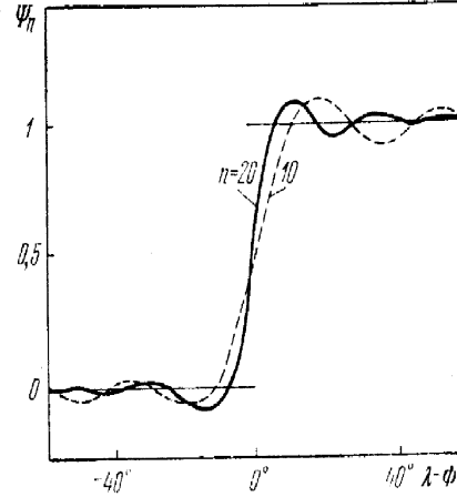
Figure 3: Vashkoviak's shadow function for upper limits of 10 and 20.
