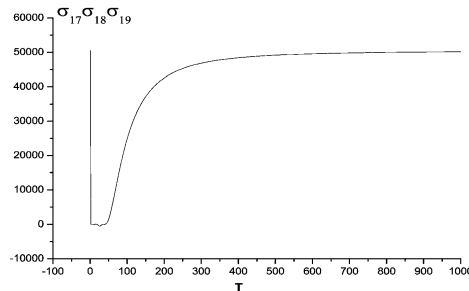
Figure 5: Amplitude multipliers \sigma_{17}\sigma_{18}\sigma_{19} .
